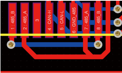
Porta BMS
